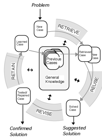
Fig. 1. CBR Cycle
